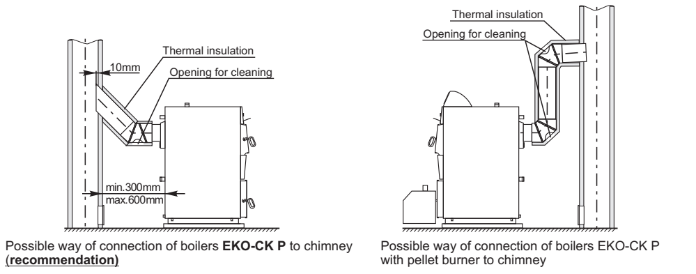
Figure 2. Possible ways of connections of boilers EKO-CK P to chimney
