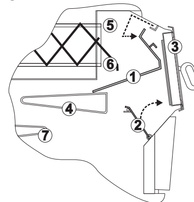
Figure 7. - Take of movable lids from combustion chamber
