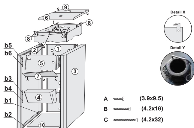
Figure 1.1. Installation of casing to boiler EKO - CK P
