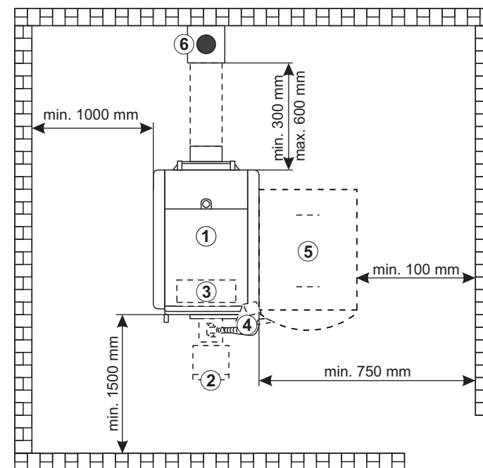
Figure 1. Minimum distance from the room walls
