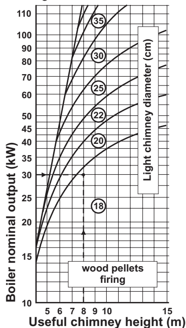
Figure 3. Chimney dimensioning for boilers EKO-CK P
