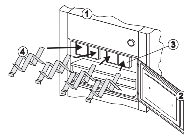
Figure 13. Mounting of turbularors
