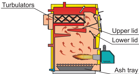
Figure 4. Movable parts of the boiler
